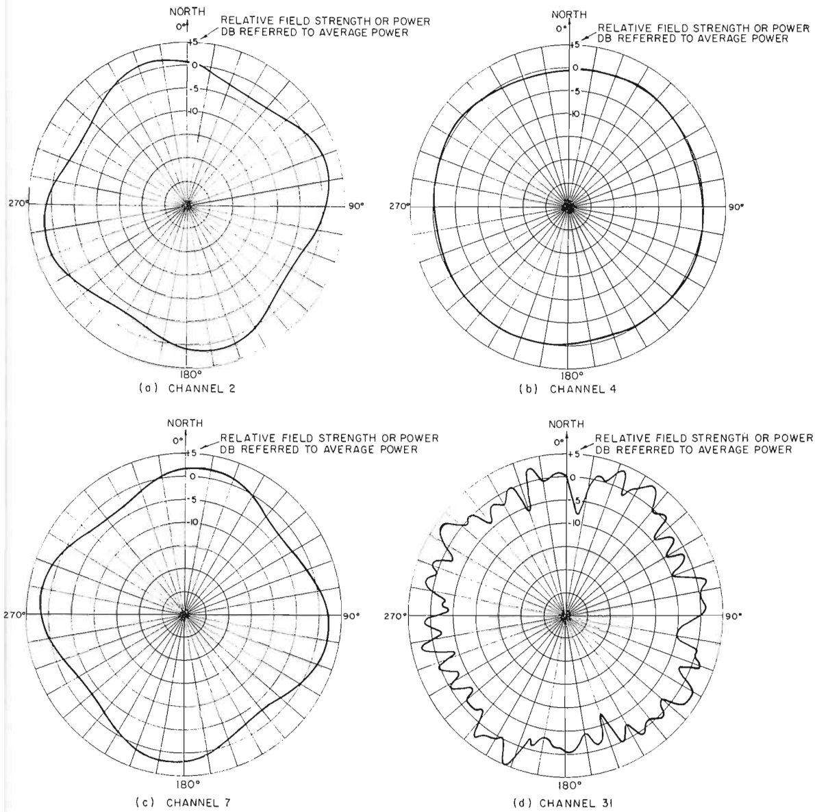
FIG. 4 TRANSMITTING ANTENNA AZIMUTH PATTERNS
