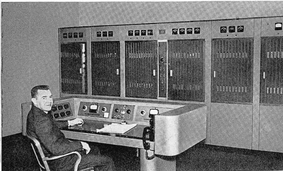
FIG. 10. The AM-transmitter facility. The cabinet at the far left houses the 1-kw (BTA-1M) nighttime transmitter and the next four house the 5-kw (BTA-5H) daytime transmitter. Cabinet at far right contains the antenna-phasing equipment. Transmitter Supervisor Roy Horsman at the console.
