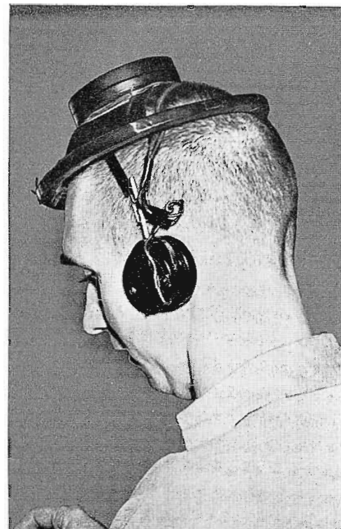
FIG. 13. WBOC-TV's "radio hat"—a station-fabricated device that permits one-way communication between control room and the studio floormen. The transistron receiver is in the 16-mm film can at the "peak" with the loop antenna in the "brim".
