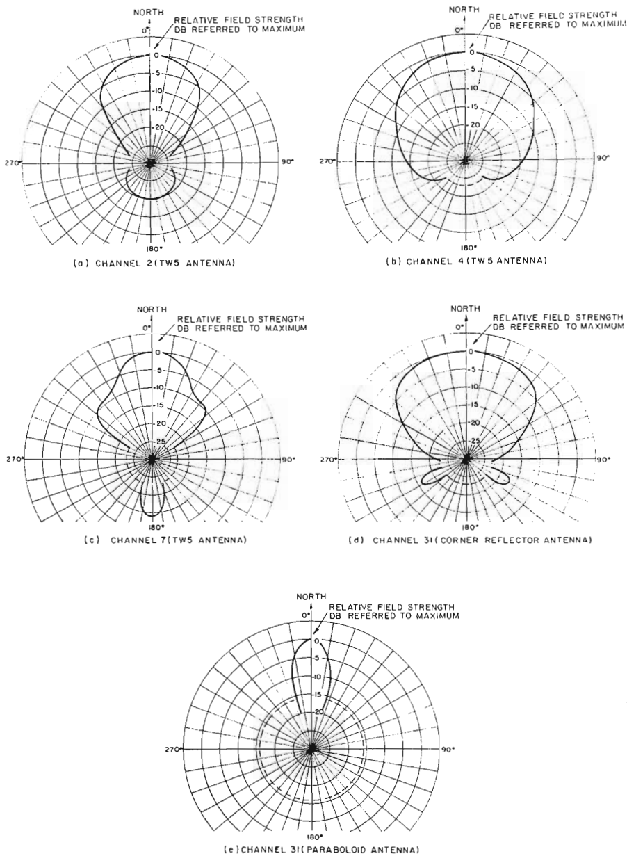
FIG. 7 RECEIVING ANTENNA AZIMUTH PATTERNS
