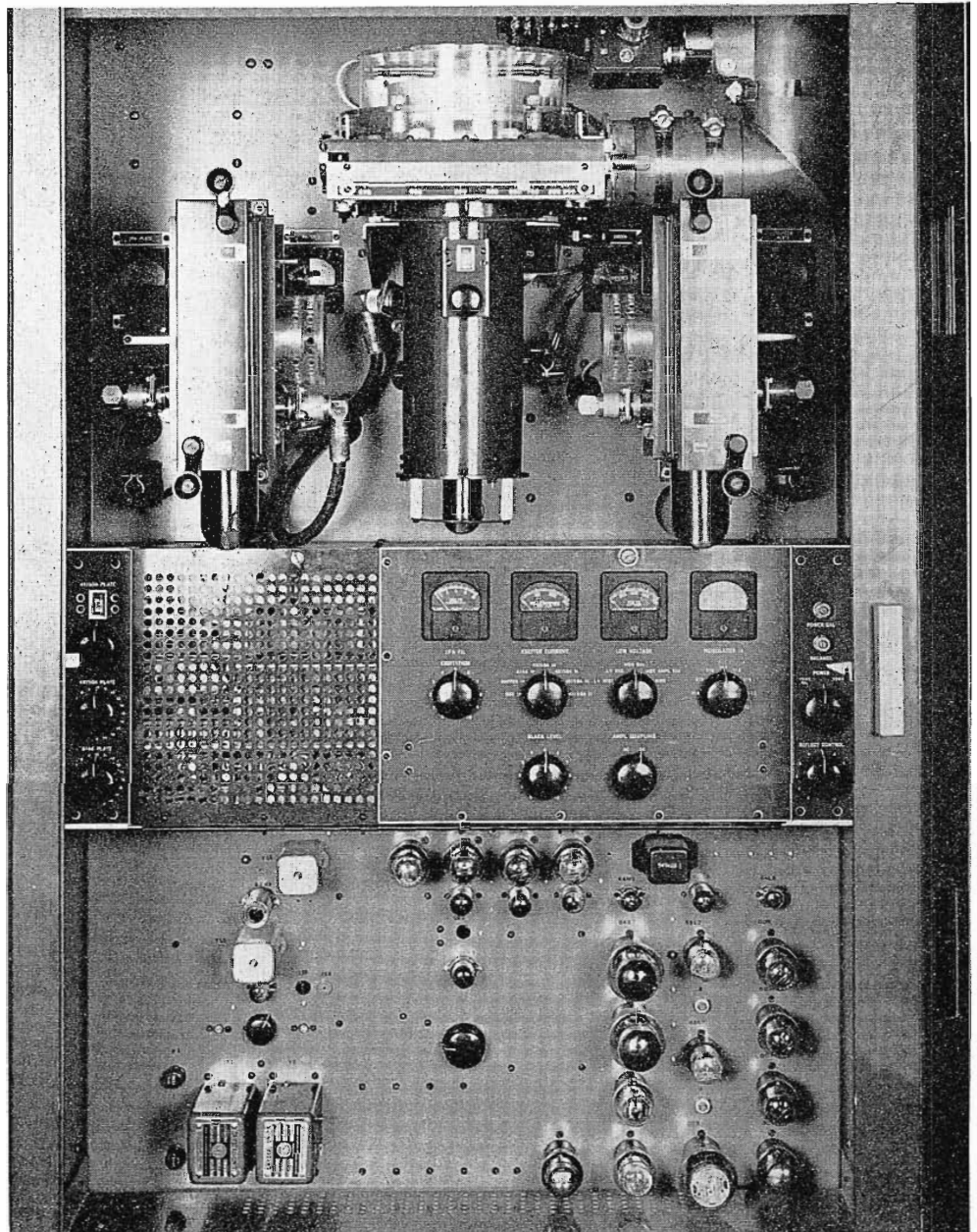
FIG. 2. Close-up of visual-transmitter panels.
