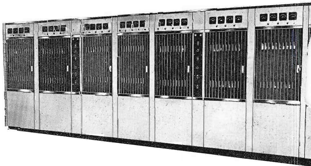
FIG. 1. Type TTU-50A 50-KW UHF Television Transmitter. With a high gain antenna can achieve effective radiated power of two million watts.
