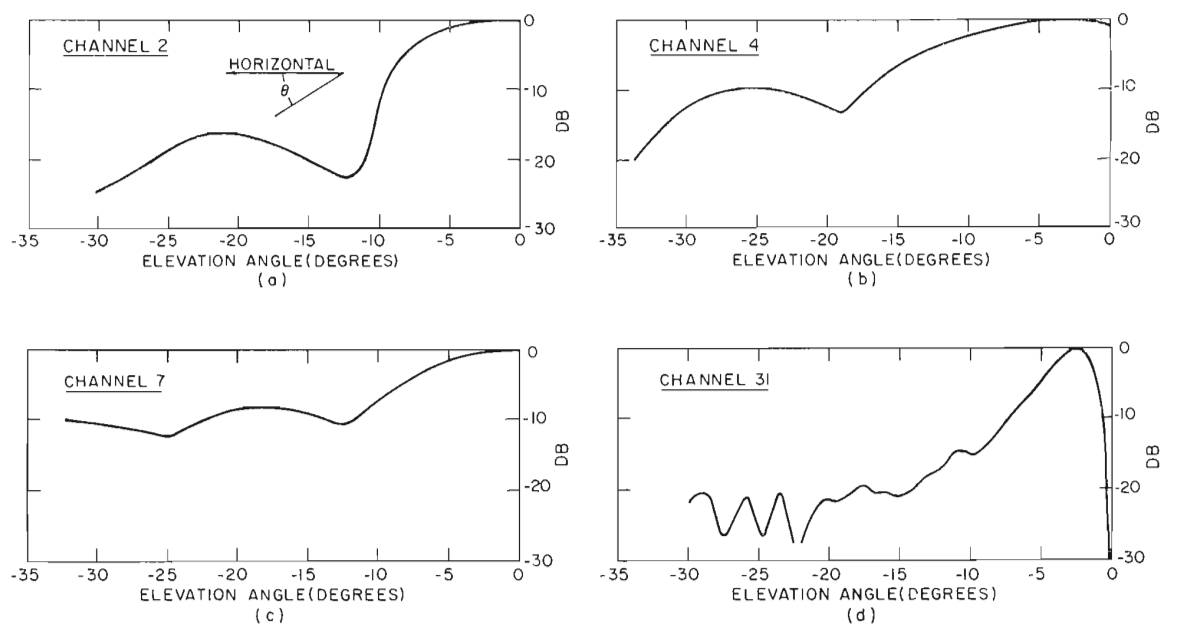
FIG. 5. TRANSMITTING ANTENNA ELEVATION PATTERNS. ORDINATE IS RELATIVE POWER IN DB REFERRED TO AVERAGE POWER ON ELEVATION PATTERN MAXIMUM.
