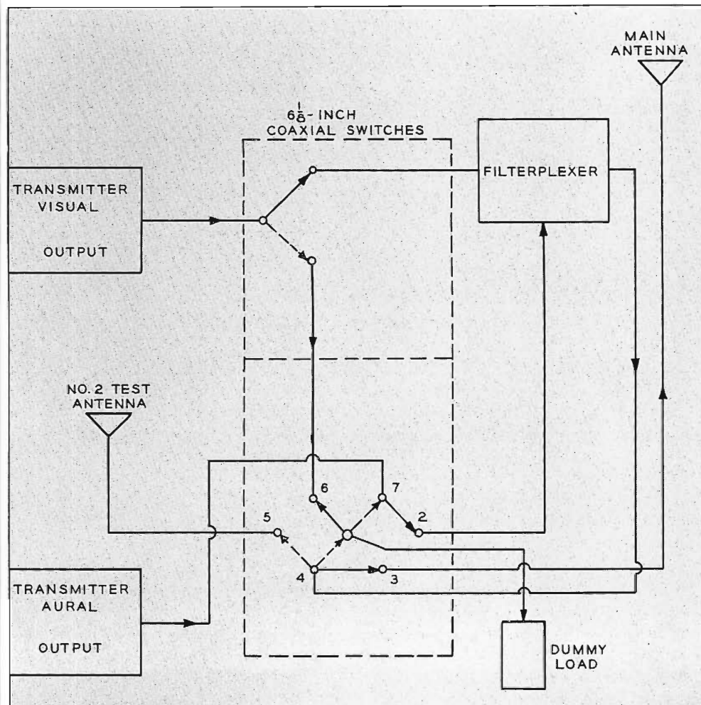
FIG. 8. Transmitter output switching circuit.
