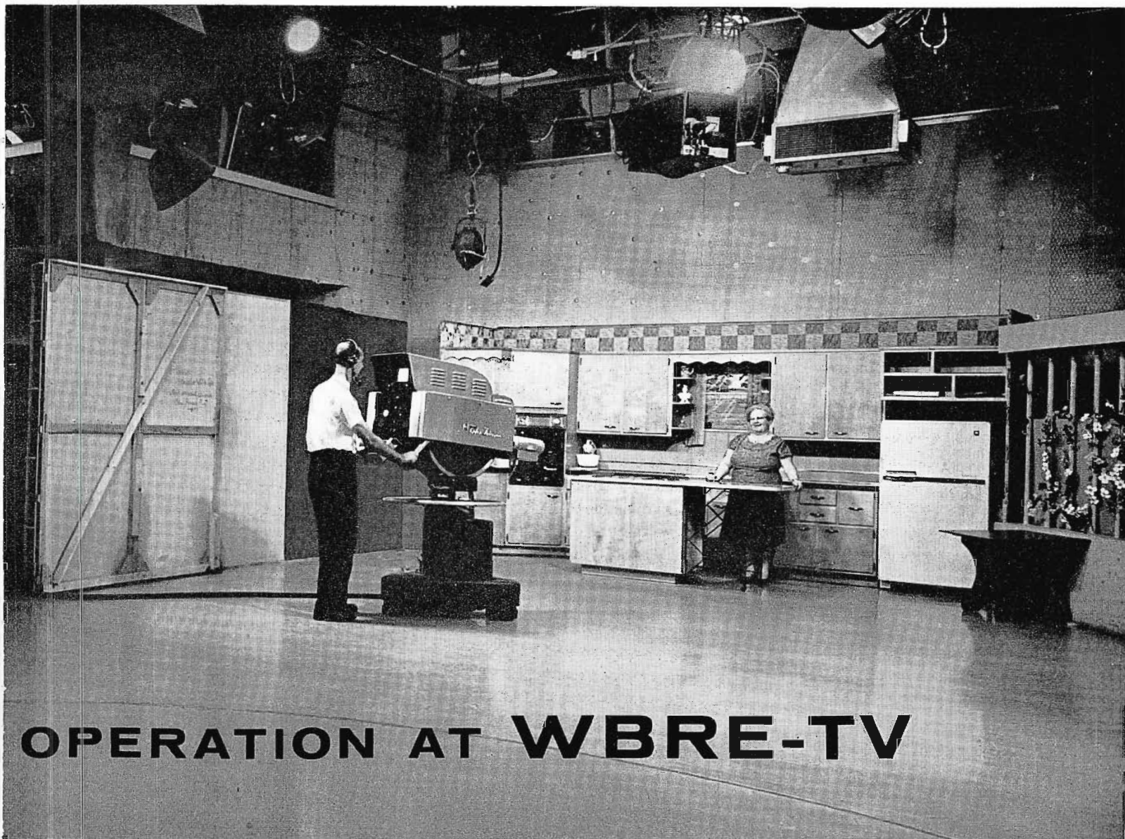
FIG. 1. Equipped for color and monochrome operations, the WBRE-TV studio typifies the modern facilities of this 10-year UHF pioneer. The studio and control room (at the upper level, overlooking the studio area) are housed in a new addition at the rear of the present location in downtown Wilkes Barre.
