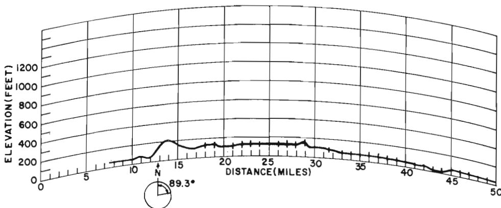
FIG. 13. ELEVATION PROFILE, EAST RADIAL (CURVATURE BASED ON 4/3 EARTH RADIUS)
