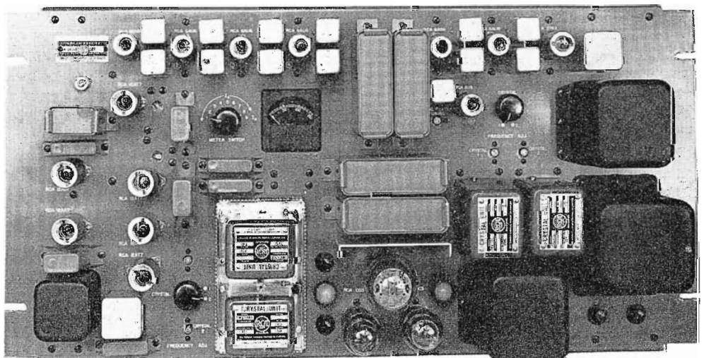
FIG. 3. Aural transmitter exciter panel.
