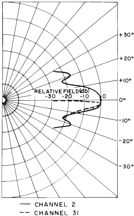
FIG. 17. TRANSMITTING ANTENNA ELEVATION PATTERNS
