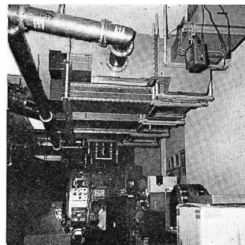
FIG. 9. Overhead installation of waveguide filterplexer.
