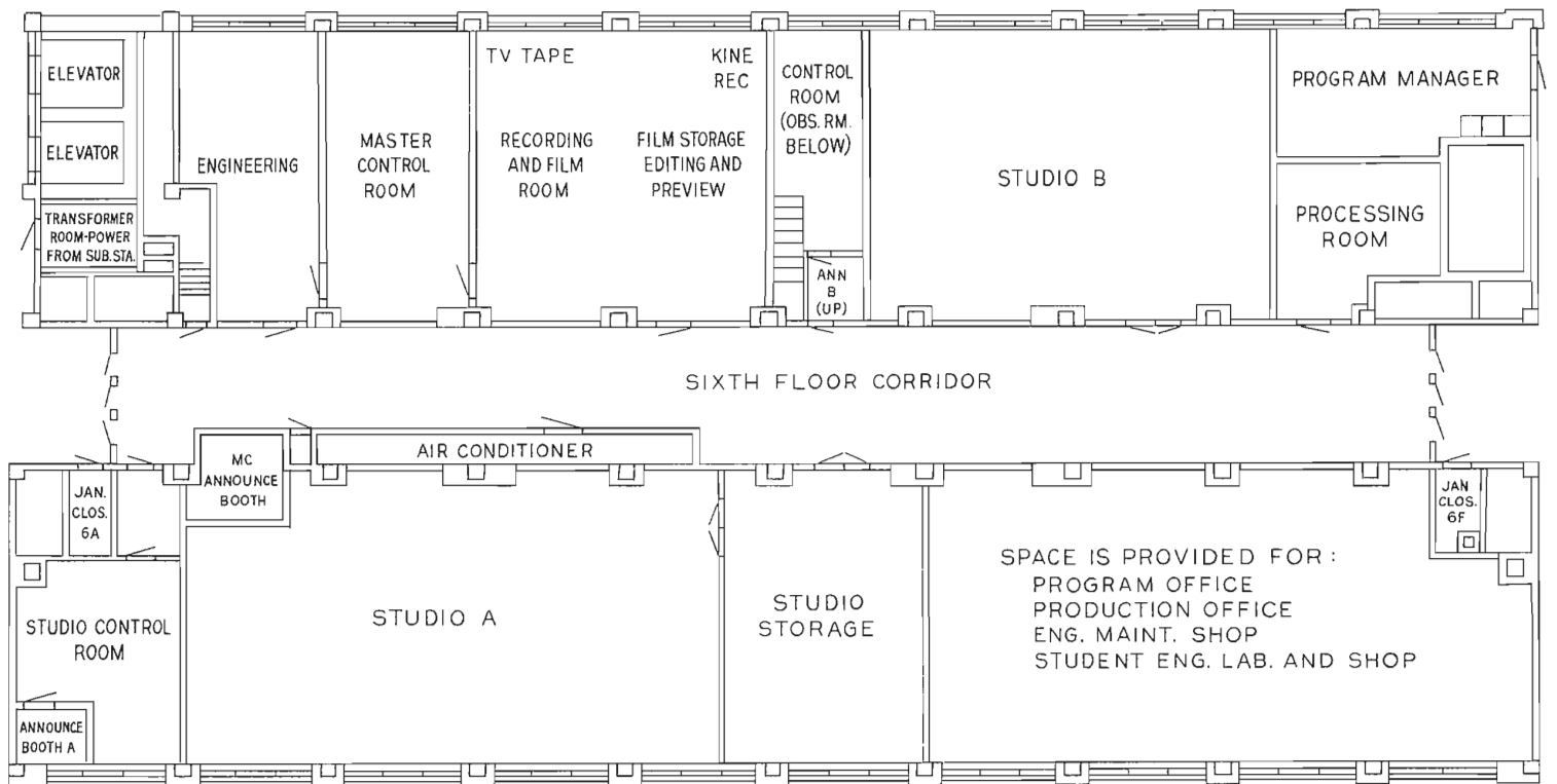
FIG. 13. Layout of ETV studio system.
