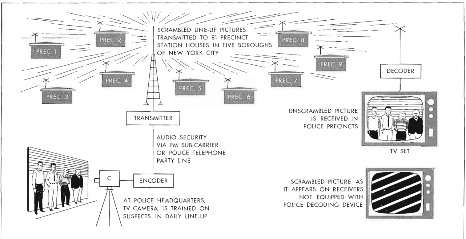
FIG. 3. System for scrambling broadcasts of police line-ups.
