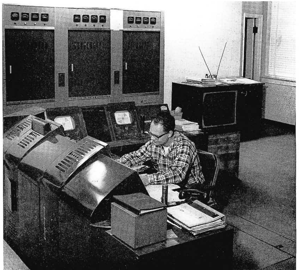
FIG. 16. UHF Television Transmitter, type TTU-1B. Transmitter supervisor, Harold Wagner is at operating console.
