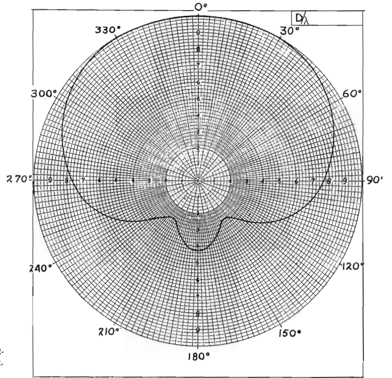
FIG. 5. Typical horizontal "Skull" pattern obtained with RCA UHF antenna.
