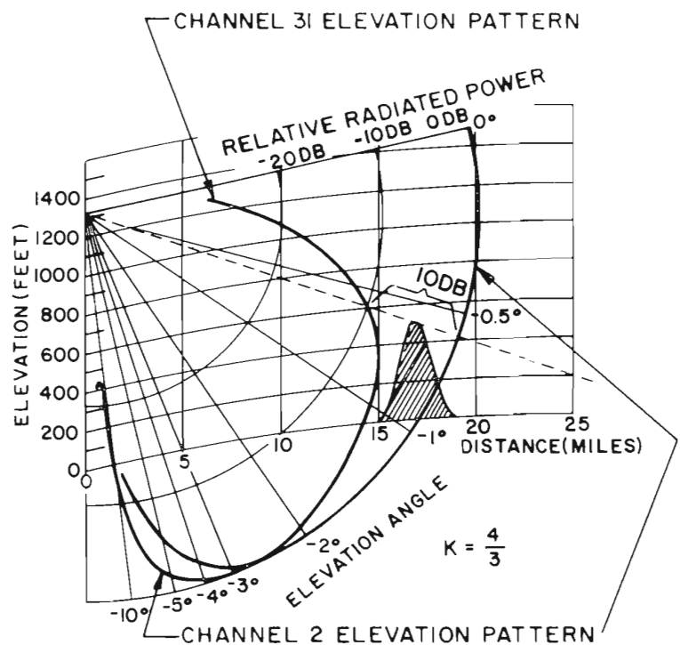
FIG. 18. ELEVATION PATTERNS SUPERIMPOSED ON SPHERICAL EARTH COORDINATES
