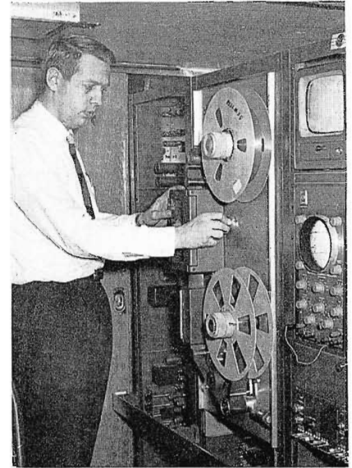
FIG. 20. Engineer Tom Brask, remote supervisor at TR-11 TV tape recorder in mobile unit. Station engineers installed the TR-11 in short racks to fit the truck.
