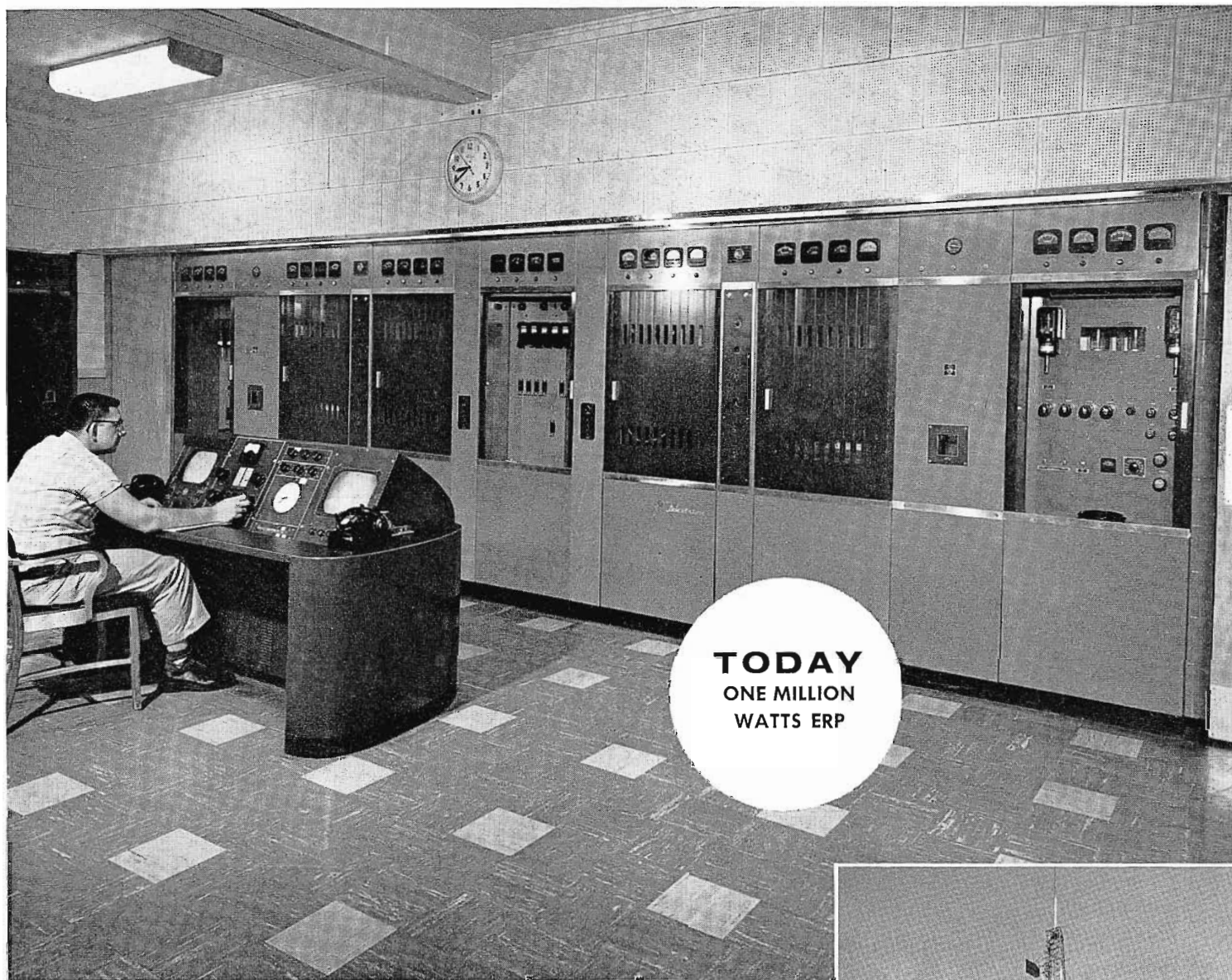
FIG. 2. TTU-25B UHF transmitter is the source of one million watts erp.
