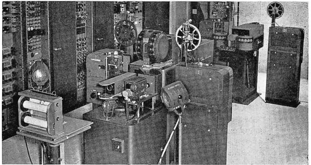
FIG. 10. Color film grouping includes all equipment necessary to originate color films, slides and opaques. A TP-15 multiplexer accommodates TK-26 color film camera, two TP-6 16-mm film projectors, TP-7 dual-drum 2 by 2 slide projector and opaque attachment.
