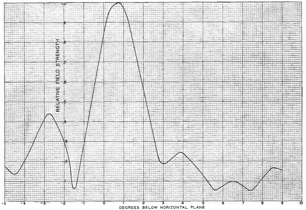
FIG. 1. TFU-24DL antenna with a 0.75 degree beam tilt. This pattern was used to obtain Curve (1) of Fig. 2. The pattern is null-filled, which means that the location of the nulls are still discernible but are filled by positive means to a given percentage. Major lobe power gain is 20.5.
