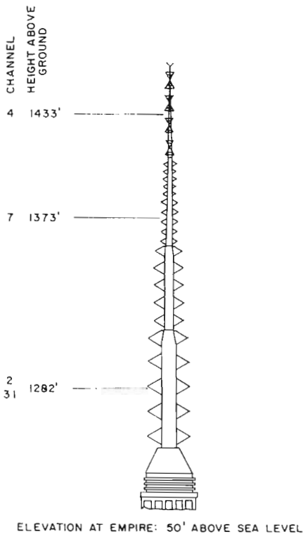
FIG. 3 EMPIRE STATE ANTENNA TOWER
