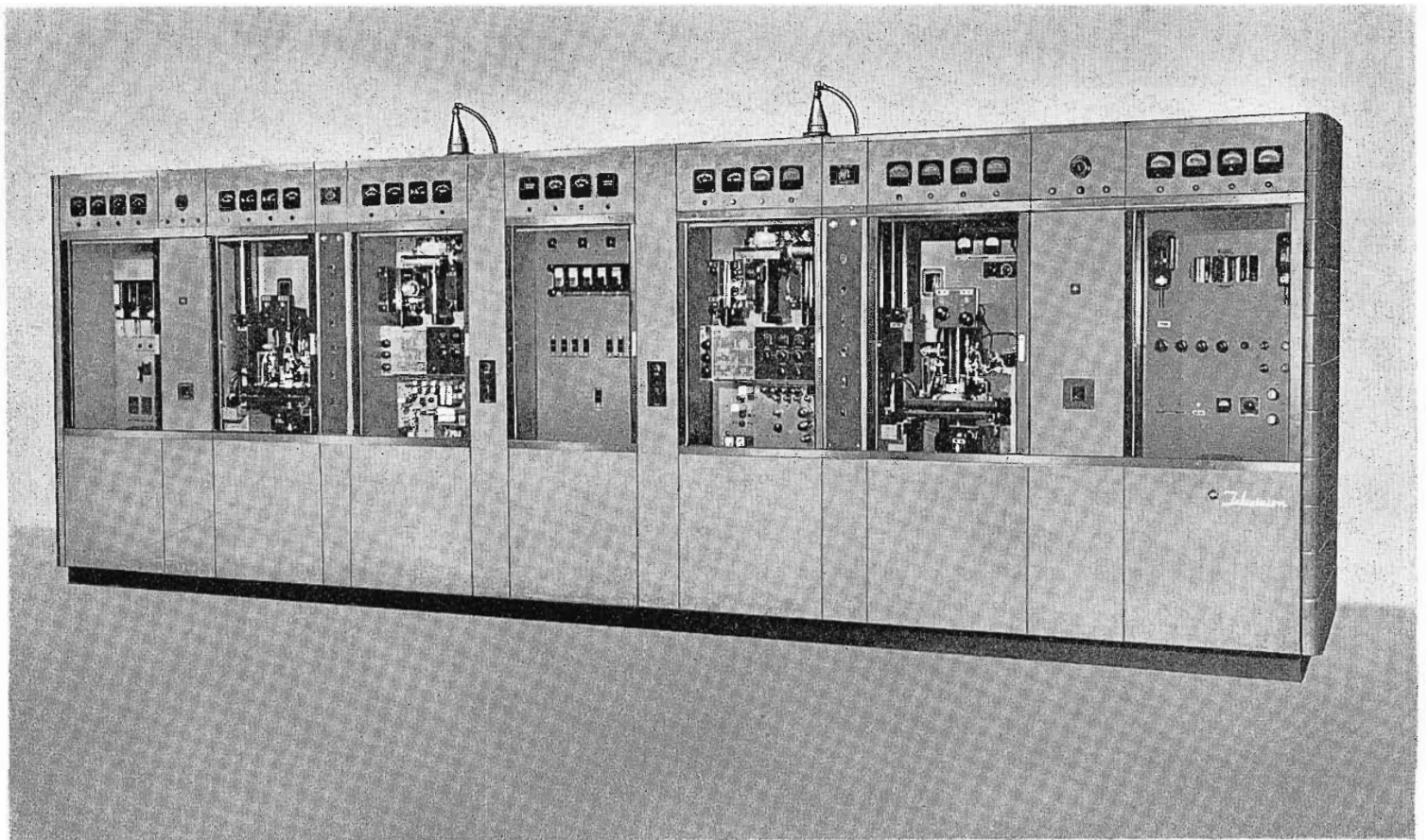
FIG. 1. The TTU-12A and TTU-25B UHF-TV Transmitter. The 12.5-kw transmitter is field expandable to 25 kilowatts without an increase in occupied floor space.
